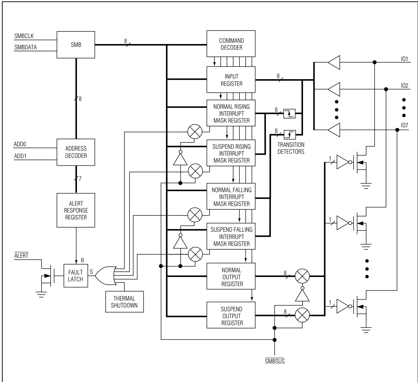
Figure 1. Functional Diagram
